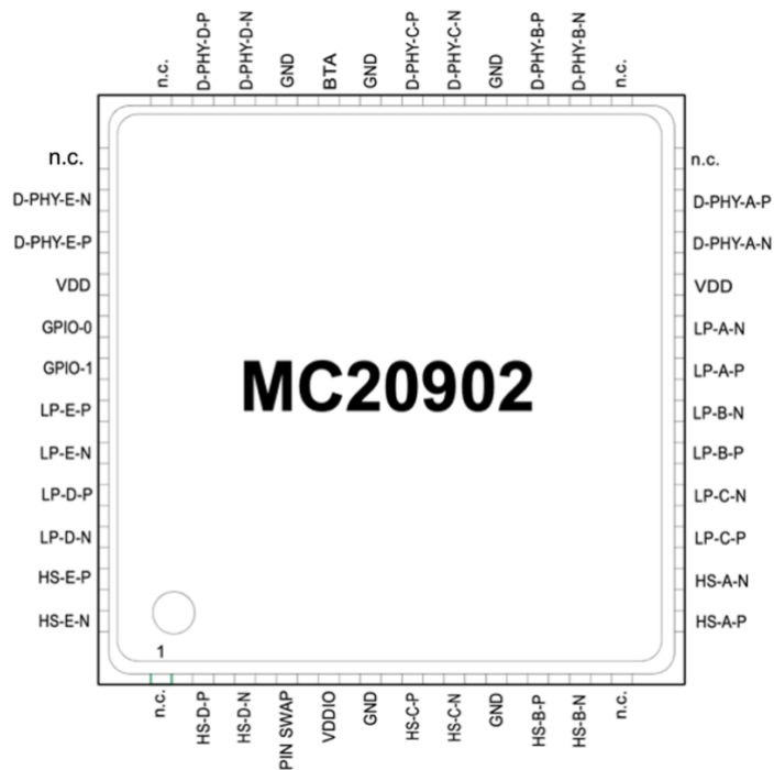
Figure 3: Pin Assignment MC20902
