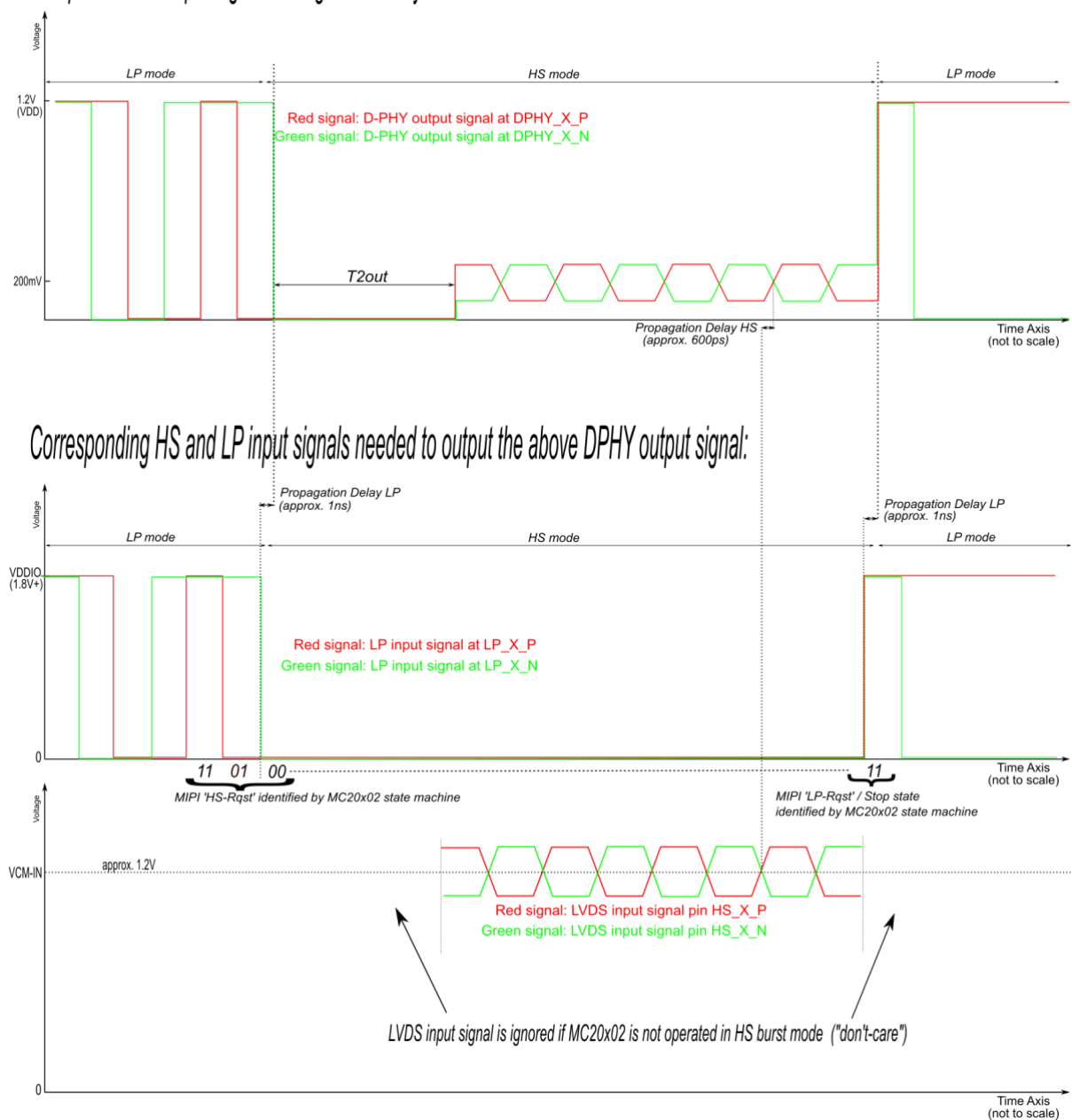
Figure 8: Input to Output Signal Diagram
